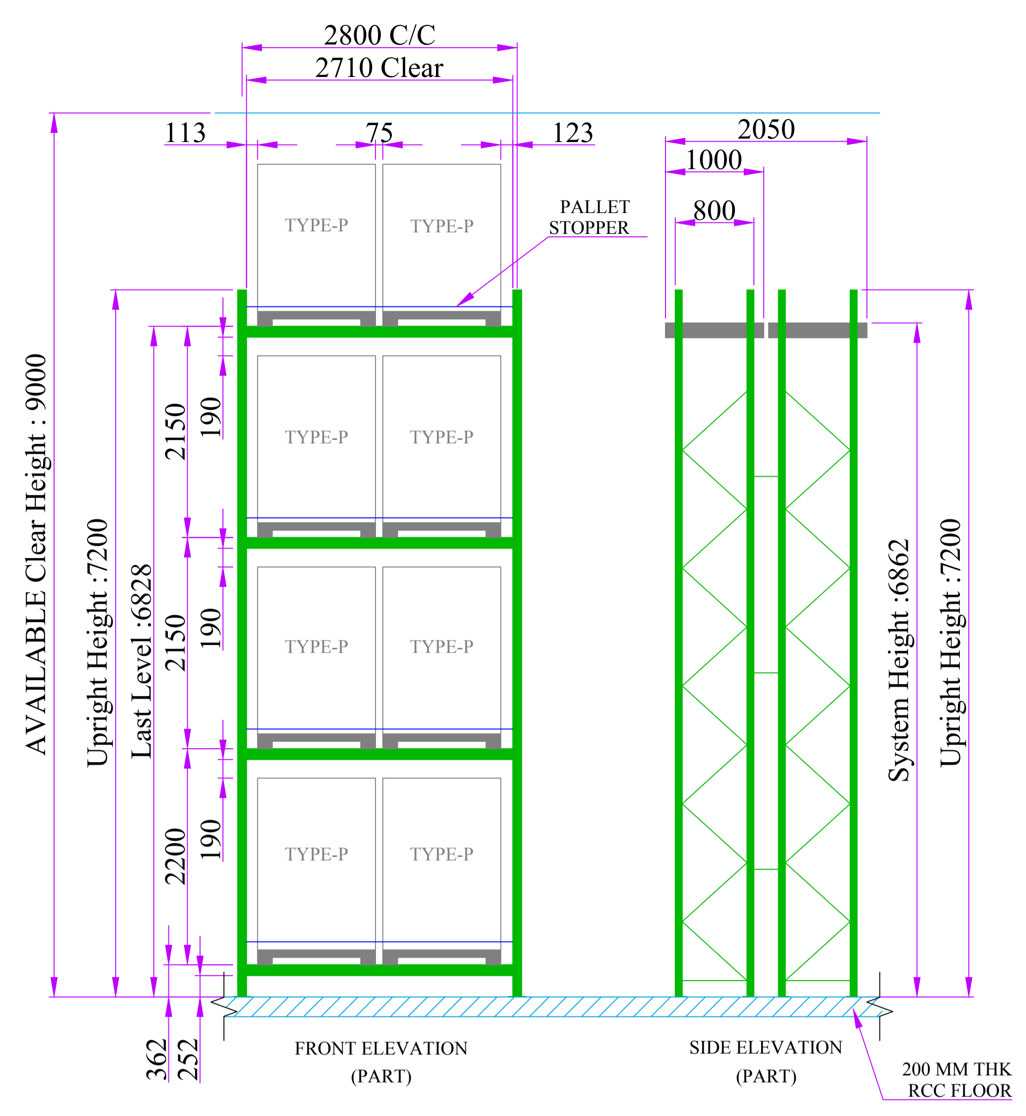
RACKS DETAILS
