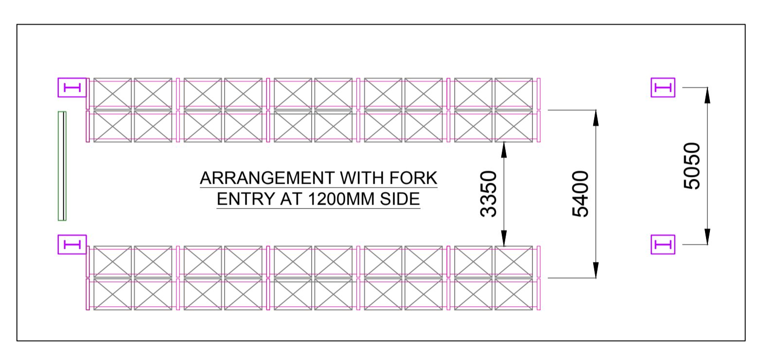
PART PLAN OF RACKING SYSTEM
