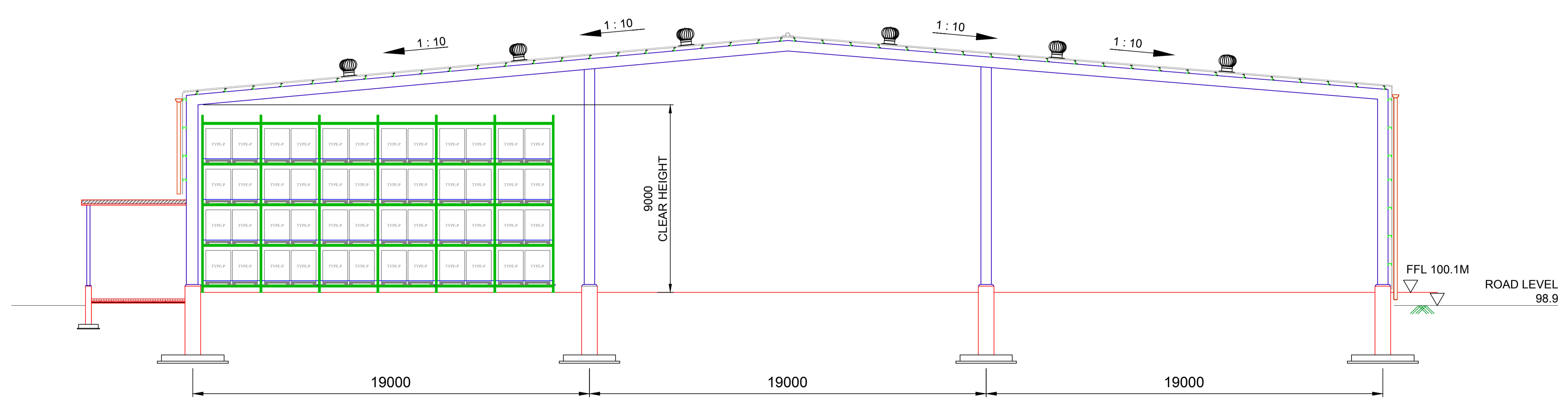
SECTION X-X
